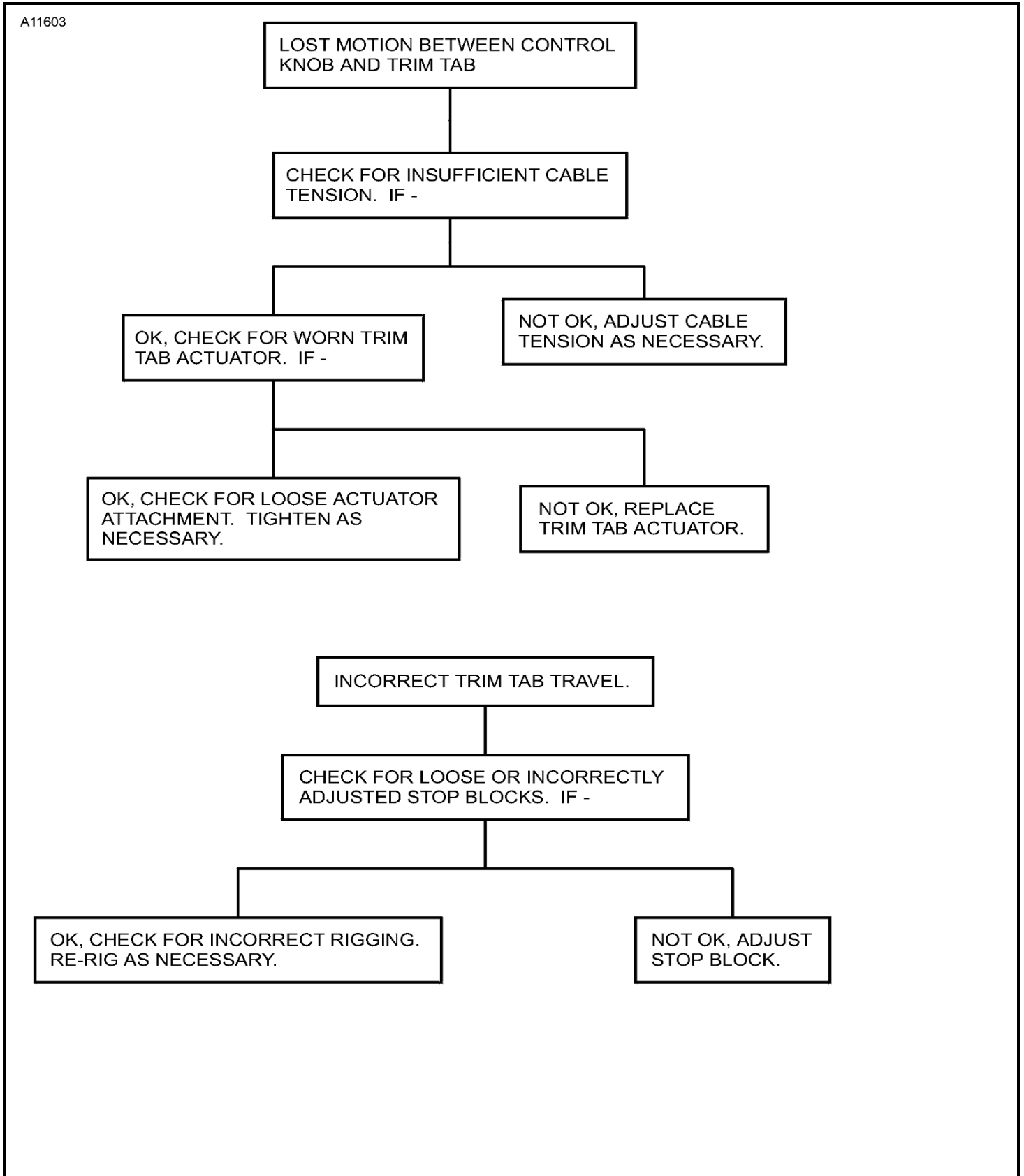
Figure 101 : Sheet 2 : Aileron Trim System Troubleshooting Chart
